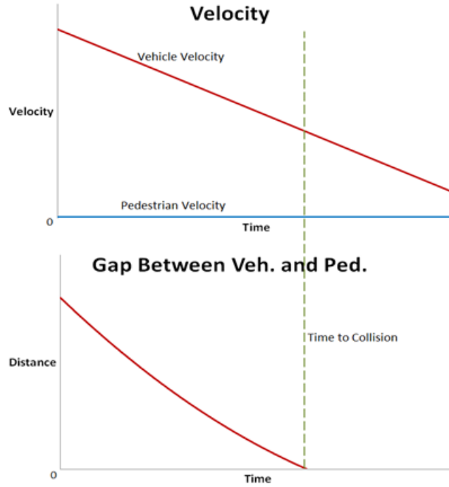
Figure 71. Vehicle-Going-Straight/Pedestrian-in-Road Timeline With Avoidance Maneuver
