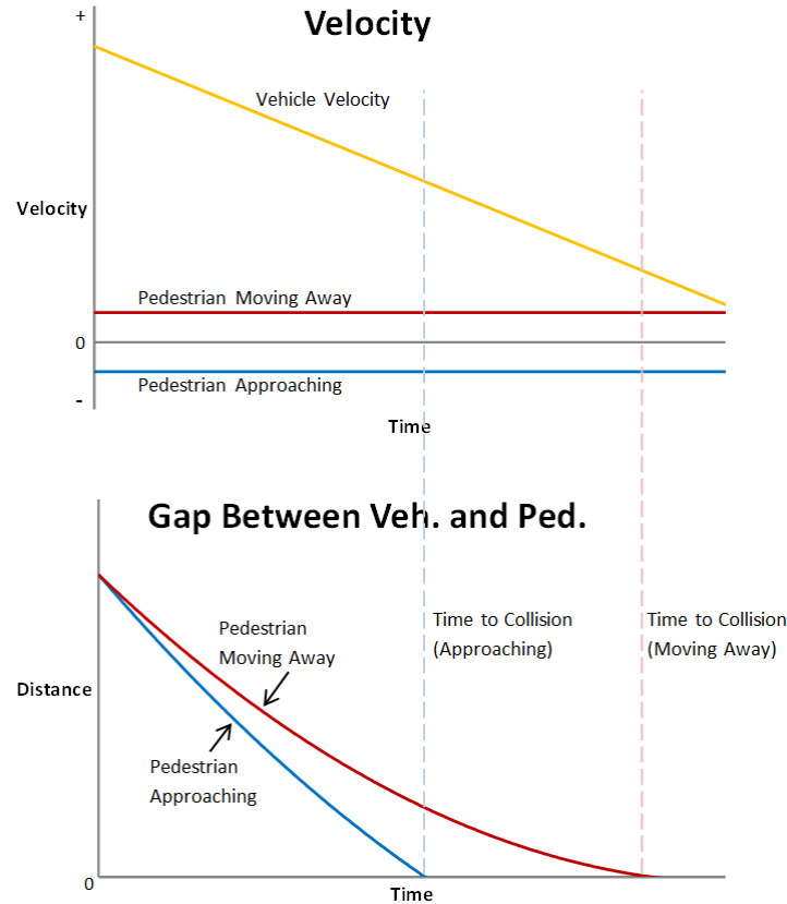
Figure 76. Timeline of Vehicle-Going-Straight/Pedestrian-Adjacent Pre-Crash Scenario With Vehicle Avoidance Maneuver
