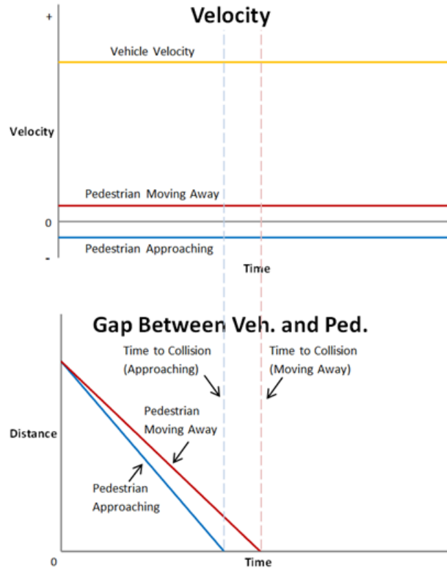
Figure 75. Timeline of Vehicle-Going-Straight/Pedestrian-Adjacent Pre-Crash Scenario
