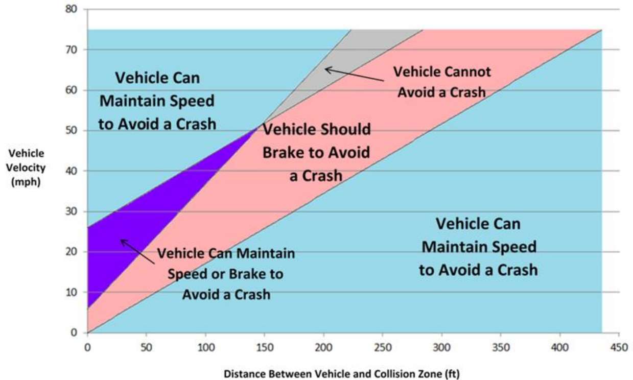
Figure 80. Distances to Avoid a Crash by Maintaining Speed or Braking (Vehicle Going Straight)
