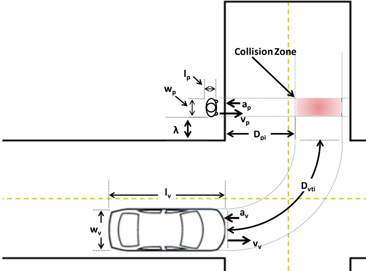
Figure 81. Vehicle-Turning-Left/Pedestrian-Crossing-Road Pre-Crash Scenario Configuration
