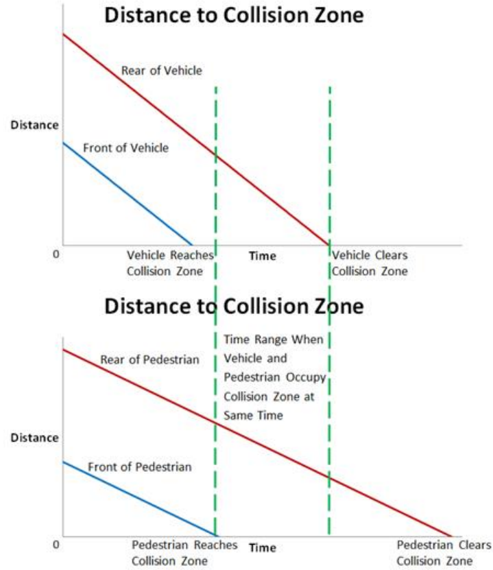
Figure 78. Timeline of Vehicle-Going-Straight/Pedestrian-Crossing-Road Pre-Crash Scenario
