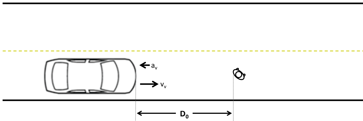
Figure 69. Vehicle-Going-Straight/Pedestrian in Road Pre-Crash Scenario Configuration
