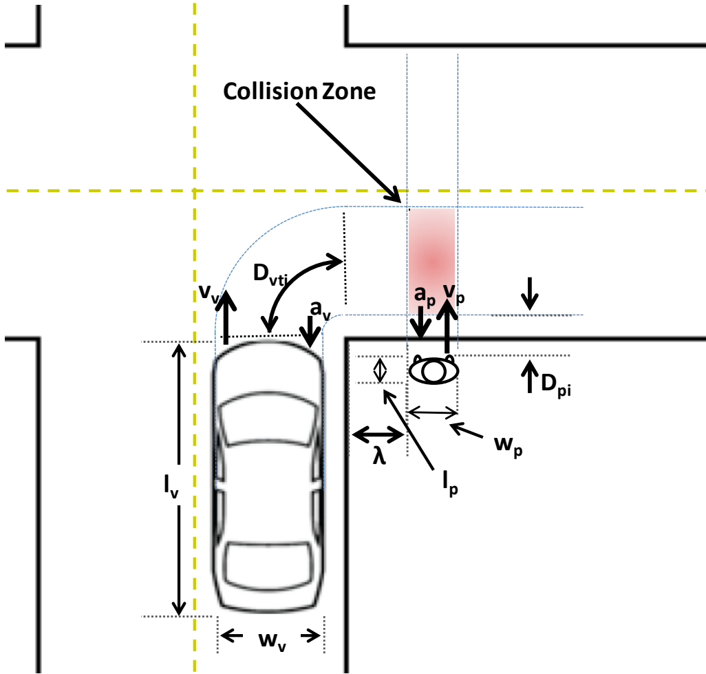
Figure 82. Vehicle-Turning-Right/Pedestrian-Crossing-Road Pre-Crash Scenario Configuration
