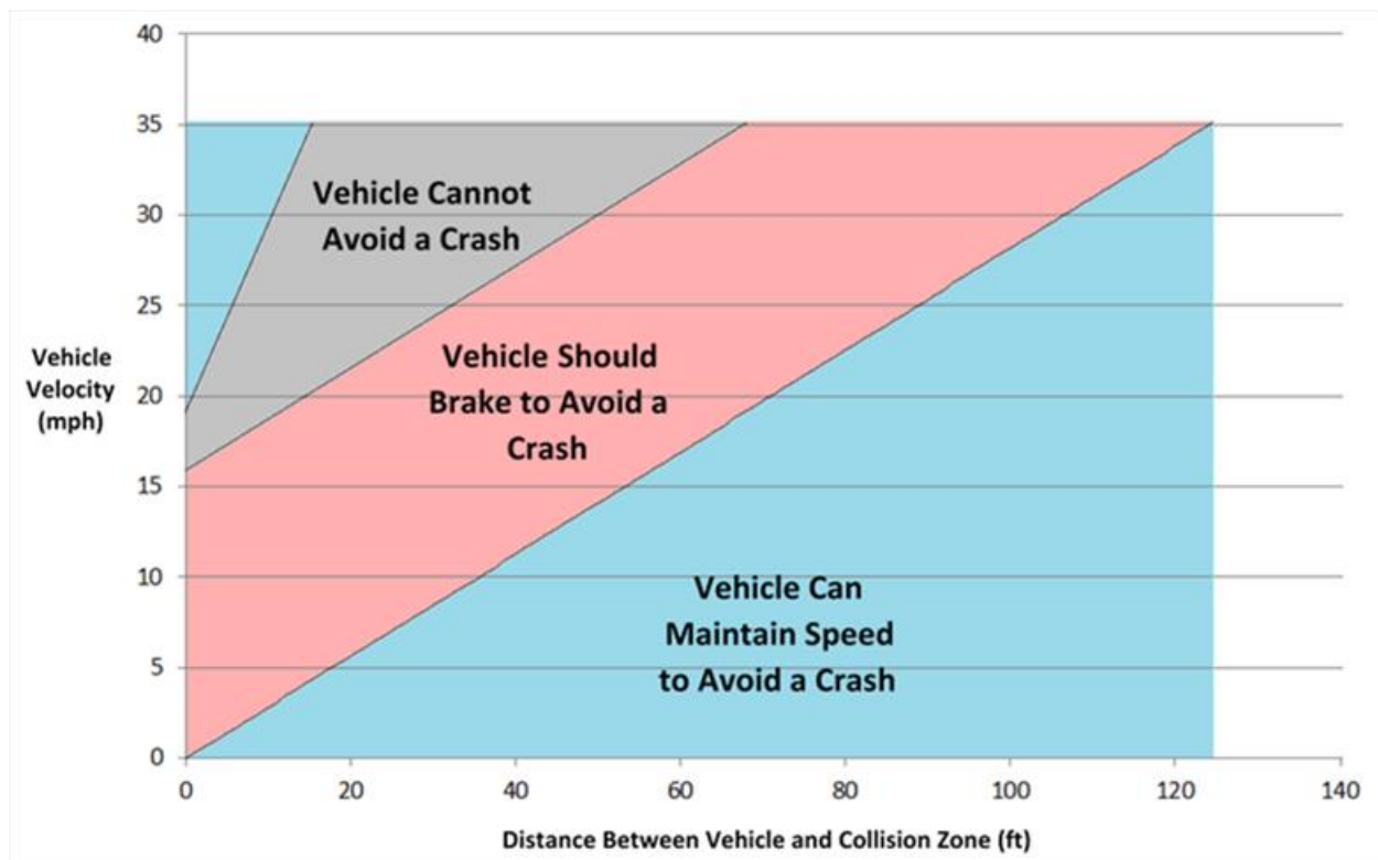
Figure 85. Distances to Avoid a Crash by Maintaining Speed or Braking (Vehicle Turning)
