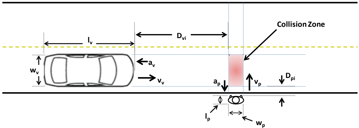
Figure 77. Vehicle-Going-Straight/Pedestrian-Crossing-Road Pre-Crash Scenario Configuration
