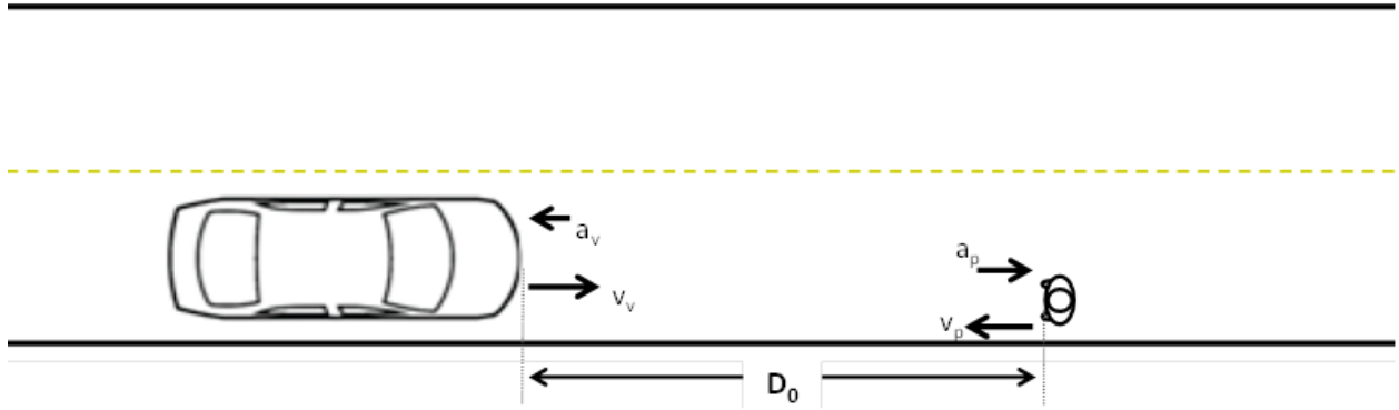
Figure 73. Vehicle-Going-Straight/Pedestrian-Adjacent-and-Approaching Pre-Crash Scenario Configuration
