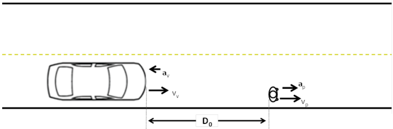
Figure 74. Vehicle-Going-Straight/Pedestrian-Adjacent-and-Moving-Away Pre-Crash Scenario Configuration
