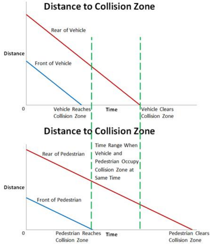
Figure 83. Timeline of Vehicle-Turning/Pedestrian-Crossing-Road Pre-Crash Scenario
