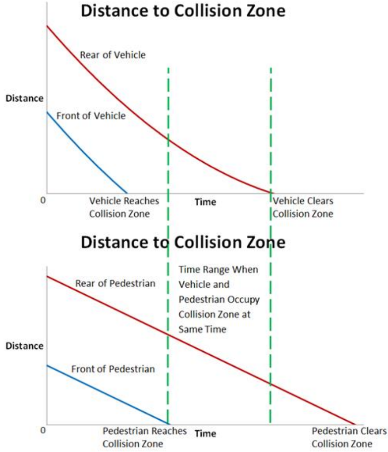
Figure 79. Timeline of Vehicle-Going-Straight/Pedestrian-Crossing-Road Pre-Crash Scenario With Vehicle Avoidance Maneuver
