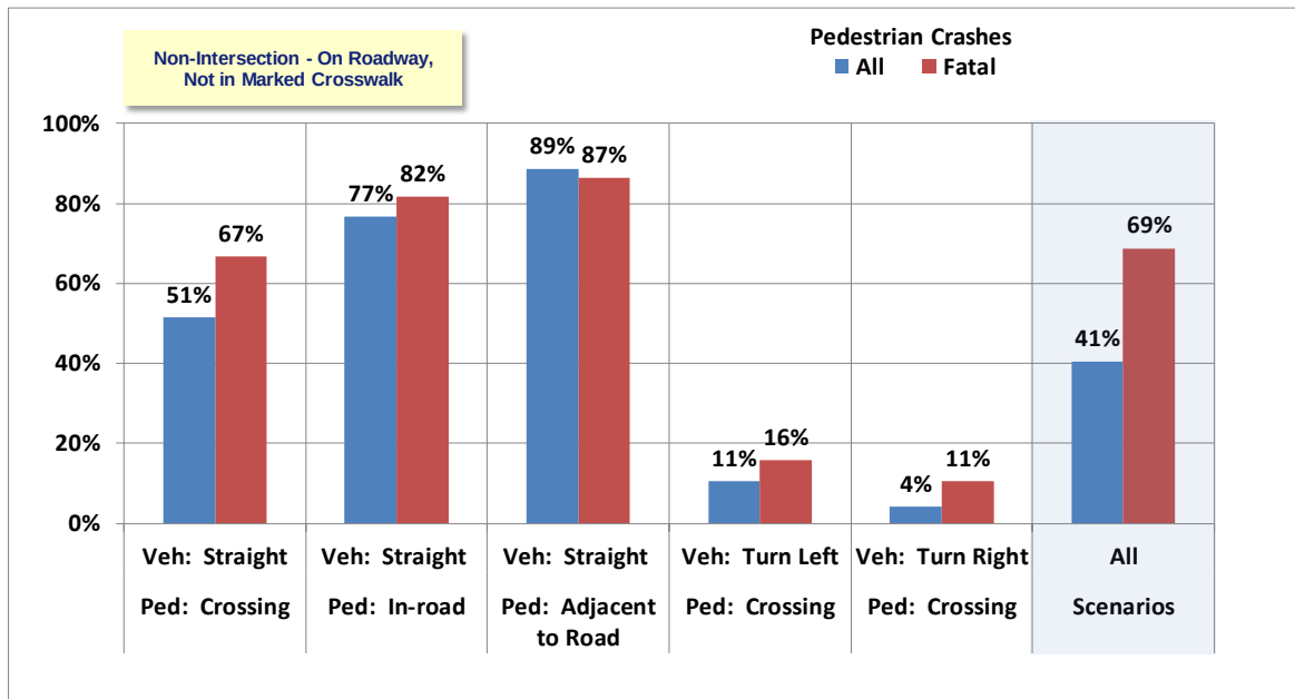
Figure 11. Percentage of “Non-Intersection - On Roadway Not in Marked Crosswalk” Crashes per Total Crashes in Each Priority Scenario
